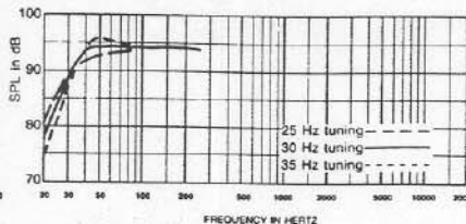
FIGURE 2B — EVX-1800 Single-Driver Low-Frequency Performance: 283-L (10-ft 3 ) Enclosure
